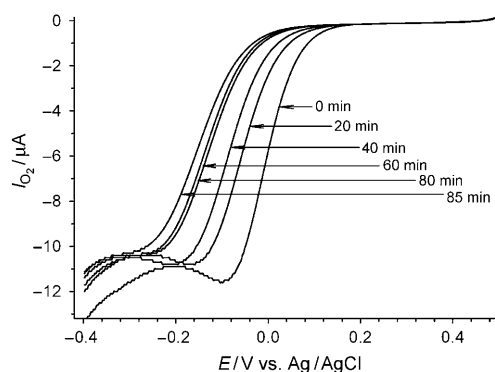
Figure 1. Voltammograms of O 2 reduction obtained in 0.1 M H 2 SO 4 after exposure of an Au electrode to Fenton’s reagent. The solution was saturated with oxygen before the experiments were carried out. Conditions: scan rate 50 mV s −1 ; gold electrode diameter ( d ) 1.6 mm; concentrations of Fe 2+ : 1 mM, EDTA: 1 mM, H 2 O 2 : 10 mM.
