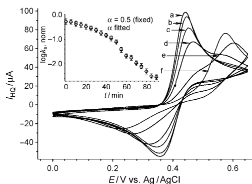
Figure 3. Cyclic voltammograms of HQ recorded in 0.1 M HClO 4 containing 100 mM NaClO 4 after exposure of the Au electrode to OH • for a) 0, b) 10, c) 20, d) 40, e) 60, and f) 90 min. Inset: Mean electron transfer rate constant of HQ versus time of reaction with hydroxyl radicals. Conditions: scan rate 10 mVs -1 ; gold electrode diameter d = 1.6 mm; c_{\text{HQ}} = 5 mM; concentrations of Fe 2+ : 1 mM, EDTA: 1 mM, H 2 O 2 : 10 mM.
